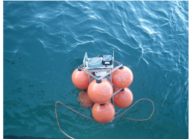
An AZFP6-ice being deployed near Nain, Labrador in October 2021. Both the AZFP and the Log IPS transducers are visible at the top of this mooring.
